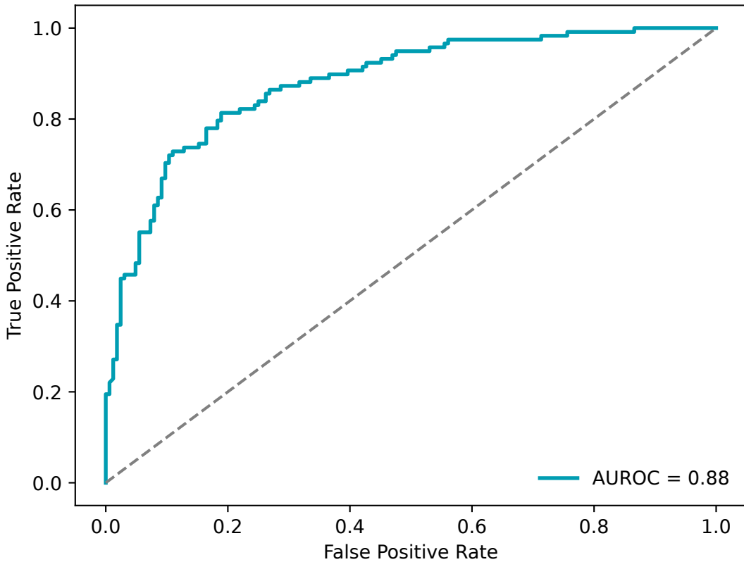
XGBOOST ROC Curve
